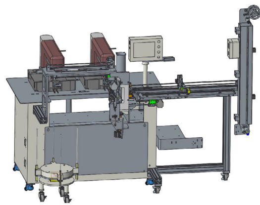
GLK-XJ2000-01 双头橡筋机 DOUBLE HEAD AUTOMATIC RING MAKE MACHINE
